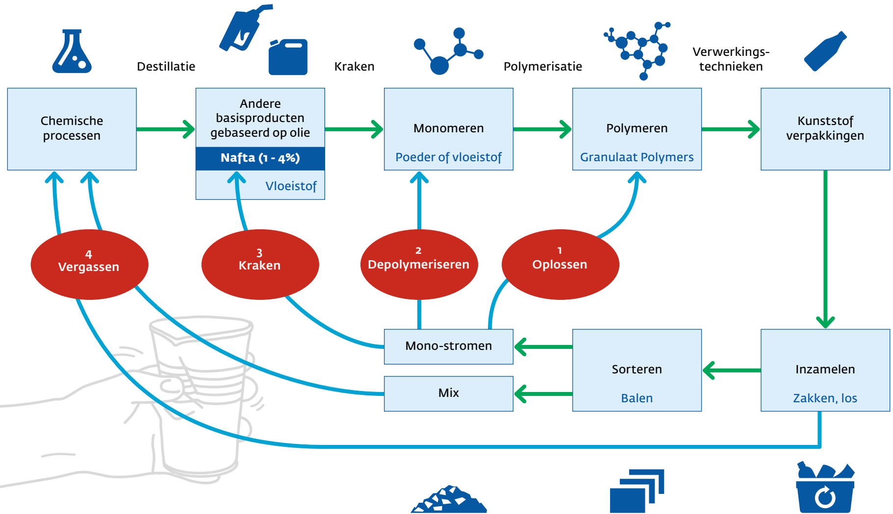
INFOGRAPHIC 15 Prototype chemische recycling kunststof (Bron: KIDV)
